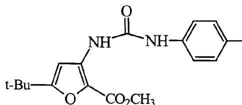
5-tert-Butyl-3-(3-p-tolyl-ureido)-furan-2-carboxylic acid methyl ester
